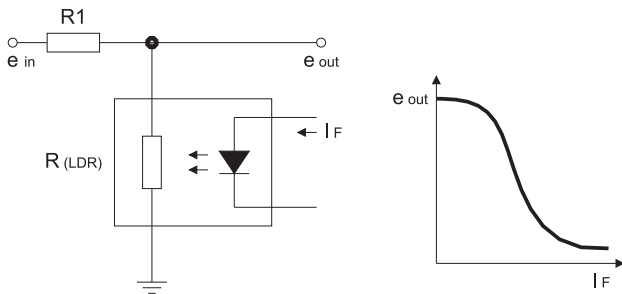
Princip paralelní regulace Principle of parallel regulation
